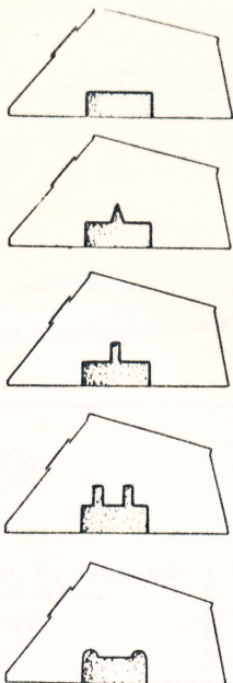
FIG. 5: This mark applies to most small-block H.P. heads beginning with '61-'63 F.I. Other applications are '66-'67 275-hp Chevy II, the '66-'67 300-hp Corvette, and '62-'64 passenger cars with H.P. option. This cylinder head marked the beginning of the large intake valve heads for small-block (1 15/16-inch intake, 1 1/2-inch exhaust in '61 to the 2.02-inch intake, 1.60-inch exhaust of later heads like current replacement head).
